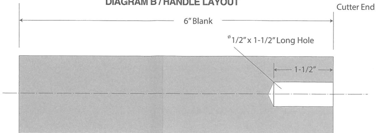
DIAGRAM B / HANDLE LAYOUT
